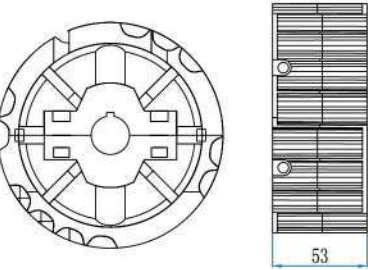
PL 812 系列 注塑主动链轮 PL 812 Series injection molded driving sprocket
